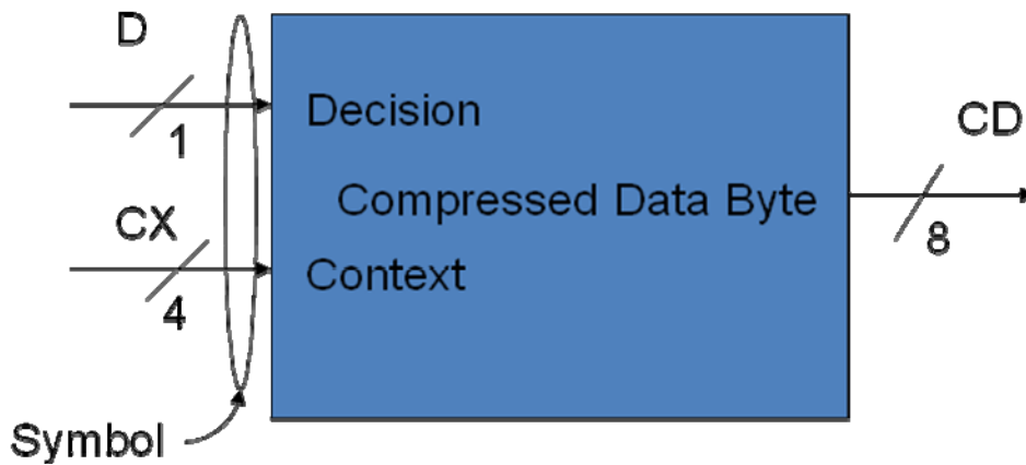
Figure 3 MQ Encoder Top Level Block
