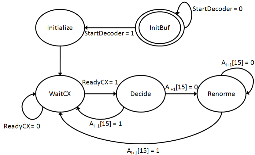
Figure 3: MQ Decoder State Diagram
