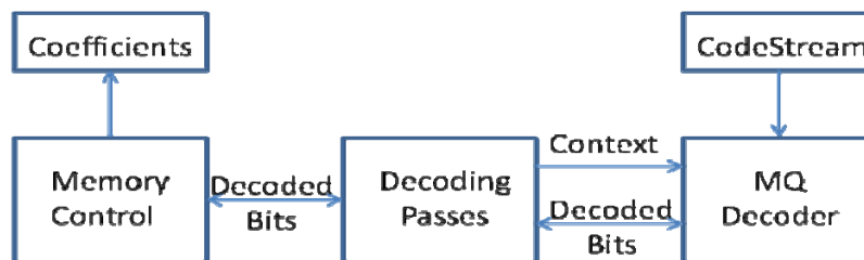
Figure 1: JPEG2000 Decoder FPGA Processing Element Overview
