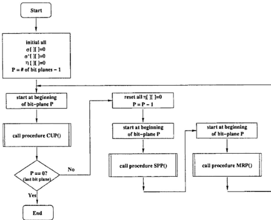
Figure 3: Top Level Flowchart for bit-plane Decoder
