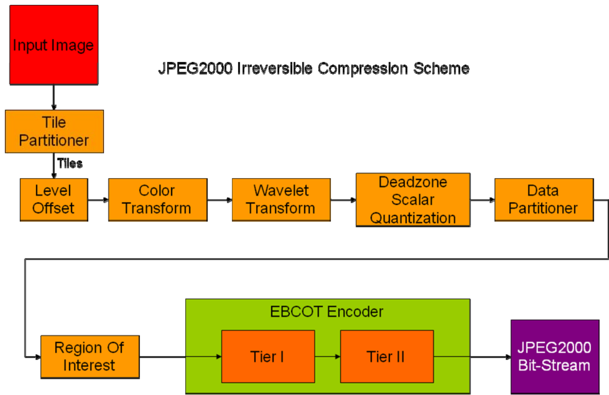
Figure 1 JPEG2000 Compression Scheme
