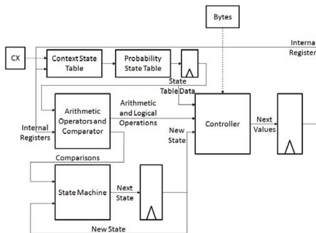
Figure 2: MQ Decoder Block Diagram
