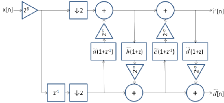
Figure 2 --- Integer based Daubechies 9/7 Transform
