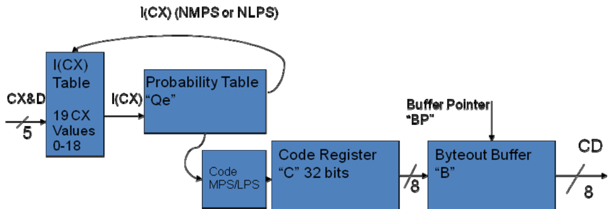
Figure 4 MQ Encoder Internal Elements
