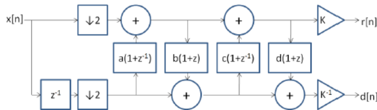
Figure 1 --- Lifting implementation of the Daubechies 9/7 Wavelet Transform
